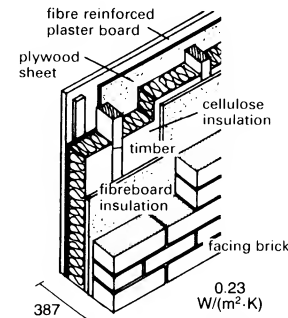
⑫ Low energy wall with facing brick 0.23 W/(m 2 ·K)
